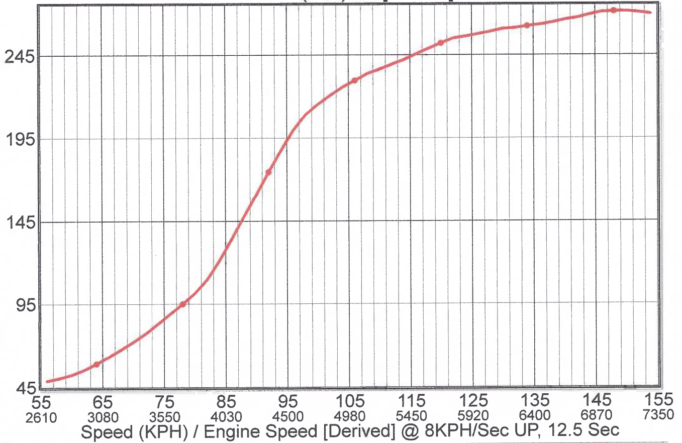
Power(KW) [ Cor'd ]
